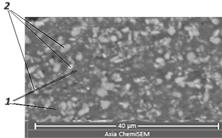
1 – \alpha - Al; 2 – \text{Al}_6\text{Fe} , \text{Al}_3\text{Fe} ( \text{Al}_{13}\text{Fe}_4 )
